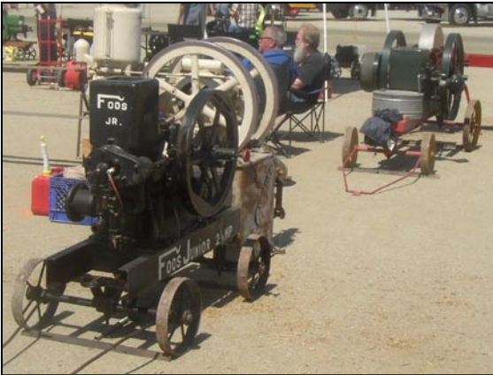
Some of Carl's other engines being set up are his 2 ½ HP 1917 Foos Jr., his 6 HP 1917 Witte and a 5 HP 1909 Stickney. All engines were running and belted to equipment at the show..... Nice set-up.
